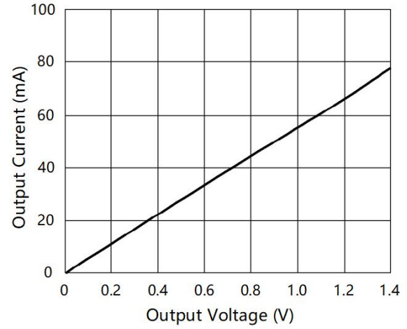
Fig.2 Output Current vs Output Voltage
