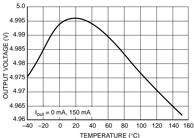
Figure 3. Output Voltage vs. Temperature (OUT = 5 V)
