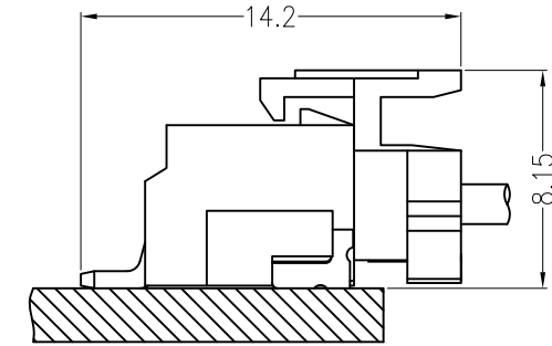
Assembly Layout
