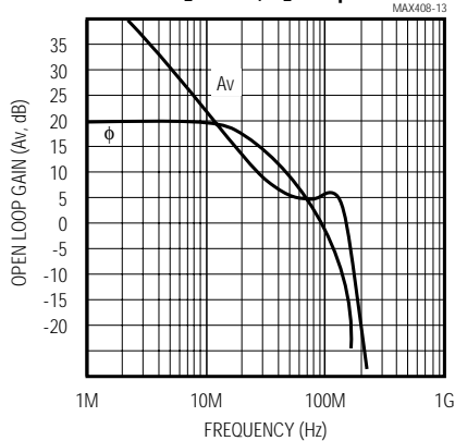
OPEN LOOP FREQUENCY RESPONSE, R_L = 2k\Omega, C_L = 50\text{pF}
