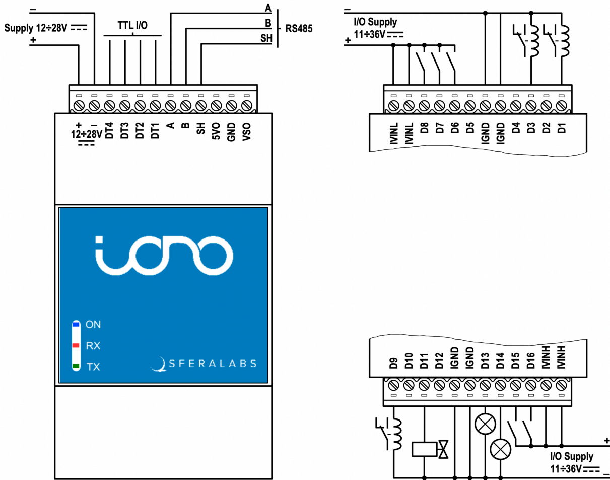
CONNECTION EXAMPLE
