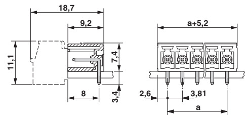
Dimensioned drawing
