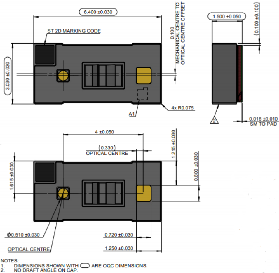
Figure 21. Outline drawing (1/4)
