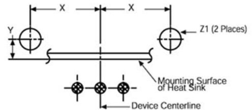
Mounting Details:
