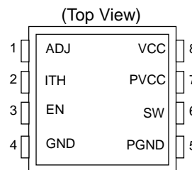
Figure 5. BD9120HFN
