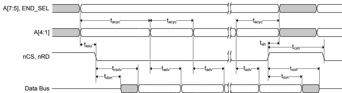
Figure 6.2 PIO Burst Read Cycle Timing
