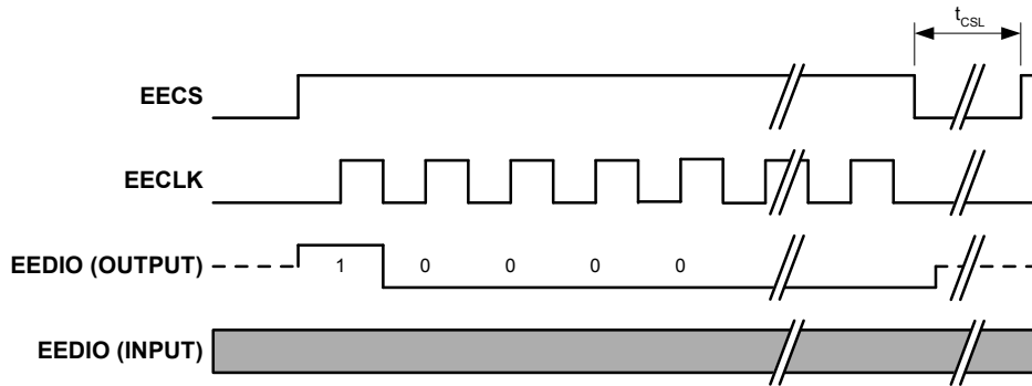
Figure 3.14 EEPROM EWDS Cycle
