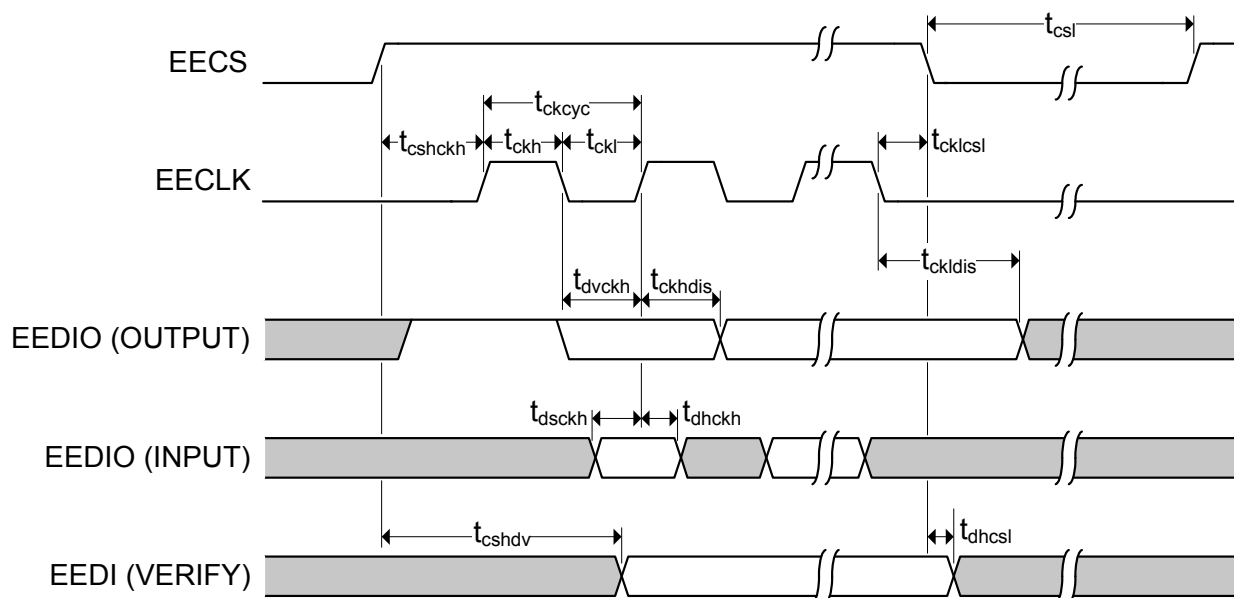
Figure 6.8 EEPROM Timing
