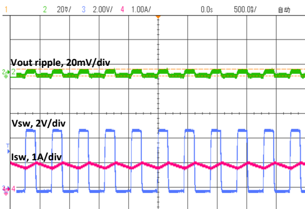
Output Ripple and SW at 1A load V_{in}=5\text{V} / V_{out}=1.8\text{V}
