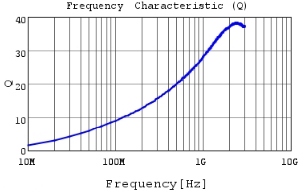
LQP03TN5N6J02 Q
