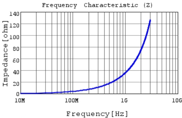
LQP03TN5N6J02 |Z|
