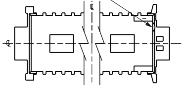
DETAIL 12 (MODIFIED DET.-1) CIRCUIT 1 LOCATION
