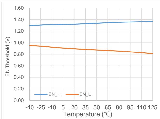
EN Threshold vs Temperature VIN = 3.3V, VOUT = 2.8V
