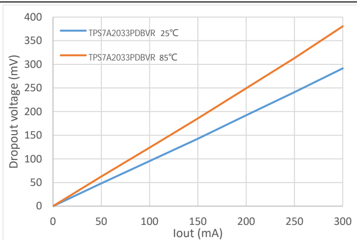
Dropout Voltage vs Output Current VOUT = 3.3V
