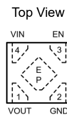
DFN1*1 Package
