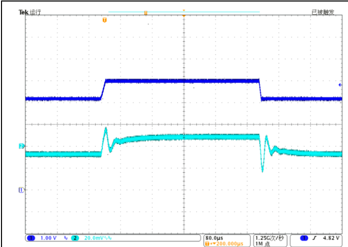
Line Transient (CH1 = VIN, CH2 = VOUT) VIN = 4.0V to 5V, VOUT = 3.3V, IOUT = 10mA
