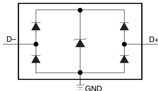
Figure 9. TPD2EUSB30/A Circuit
