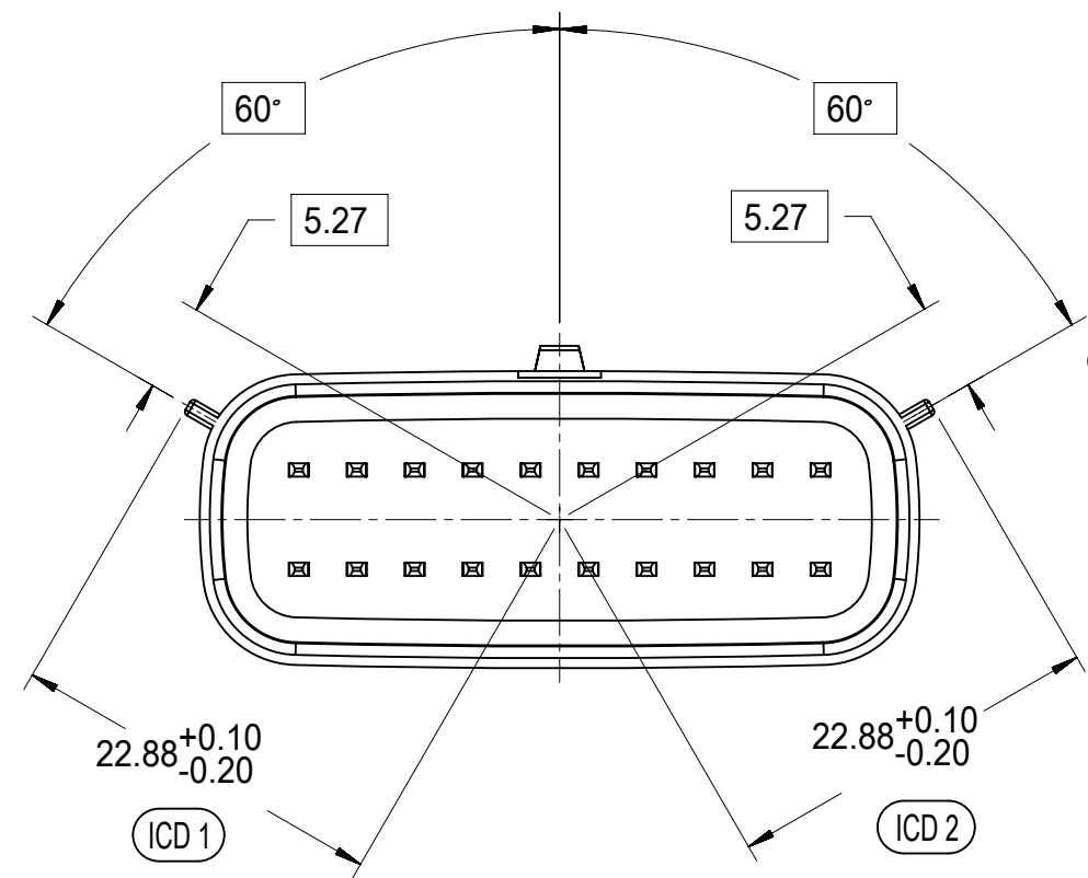
KEYING OPTION A SCALE 4:1
