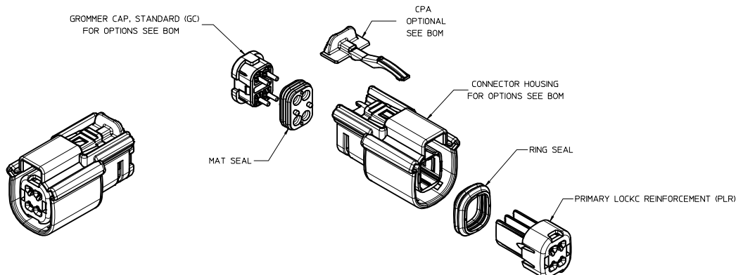
MX150 2X2 RECEPTACLE SEALED ASSEMBLY - STANDARD (STD)
