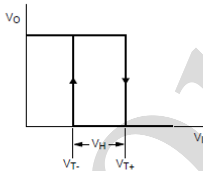
Figure 6. Transfer characteristic
