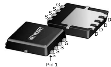
DFN5X6-8L (TDSO-8-EP(5x6))
