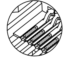
Correct soldering
