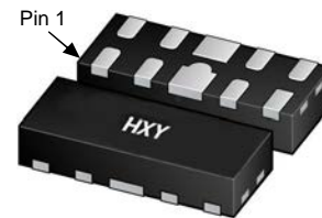
DFN2510-10L
