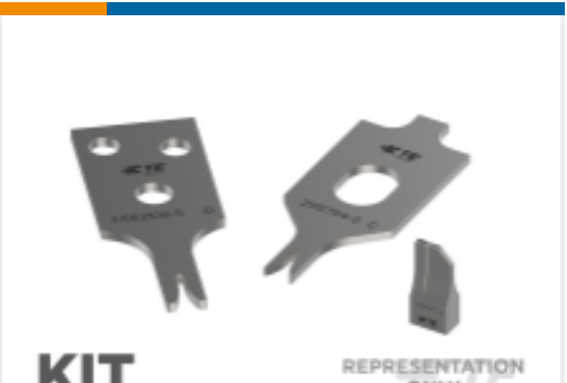
TE Part # 7-2151268-7 OCEAN_2.0_SPARE_PART_KIT-062F155O
