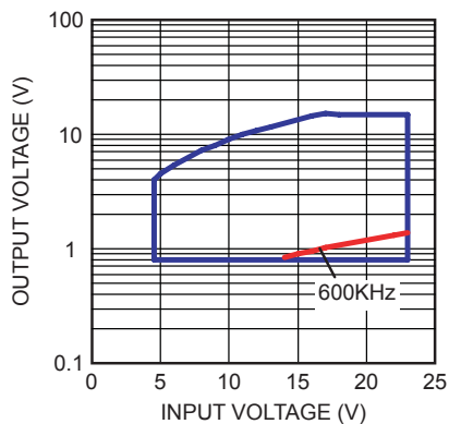
Operating Range
