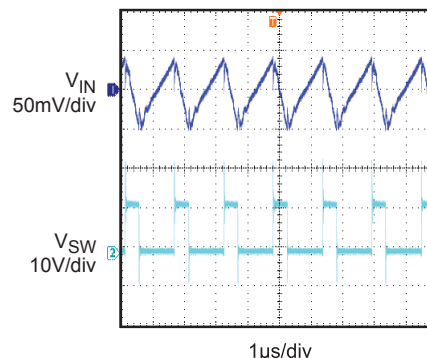
Input Ripple Voltage I_{OUT}=3A
