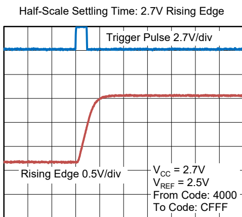
Time (2μs/div)
