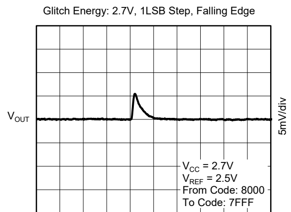
Time (2μs/div)
