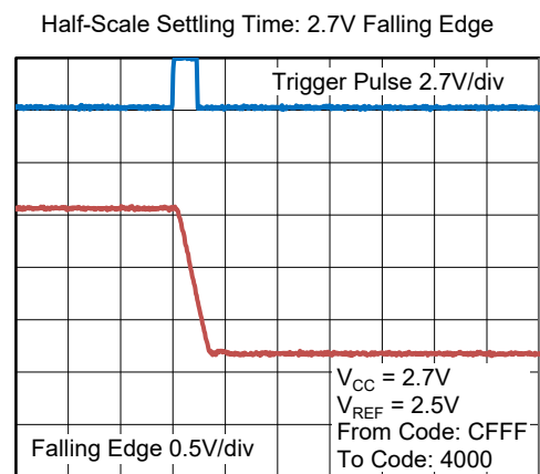
Time (2μs/div)
