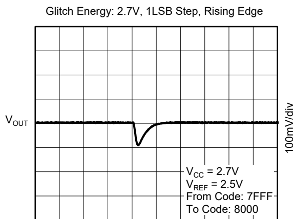
Time (2μs/div)
