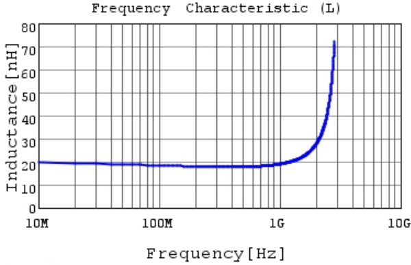
LQP03TN18NJ02 L
