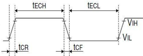
Figure 4: ZED-F9P high precision receiver UART timing specifications
