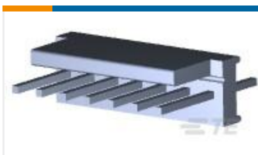
TE Part #640454-7 07P MTA100 HDR ASSY SQ STR POL
