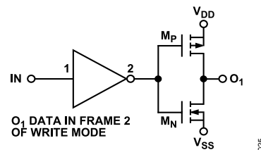
Figure 34. Output Stage of Logic Output, O 1
