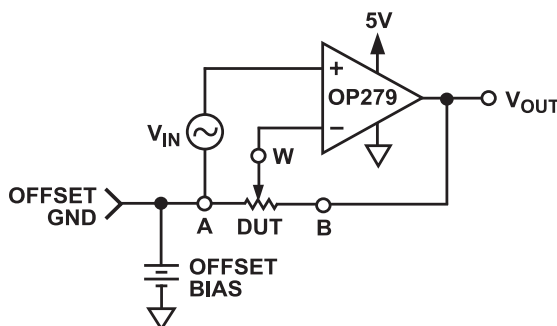
Figure 27. Noninverting Gain
