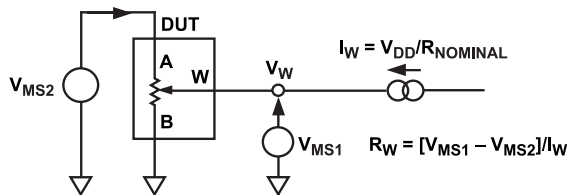
Figure 24. Wiper Resistance
