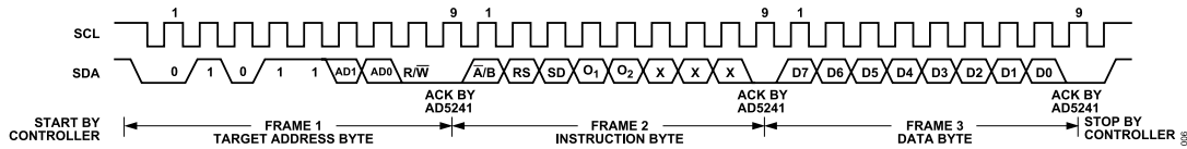
Figure 4. Writing to the RDAC Serial Register
