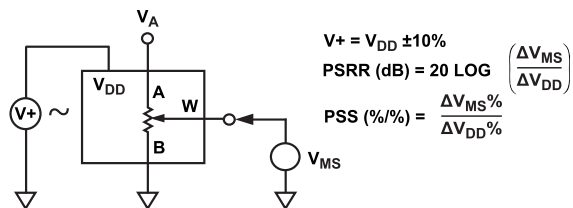
Figure 25. Power Supply Sensitivity (PSS, PSRR)
