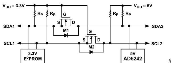
Figure 33. Level-Shift for Different Voltage Devices Operation
