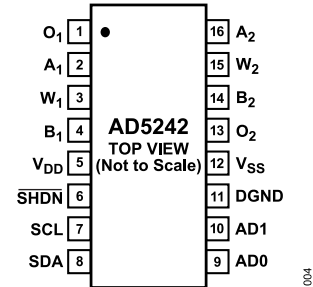
Figure 7. AD5242 Pin Configuration
