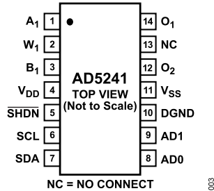
Figure 6. AD5241 Pin Configuration
