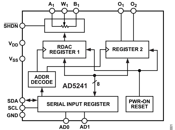
Figure 1. AD5241 Functional Block Diagram
