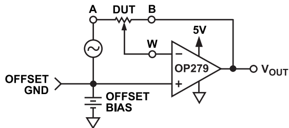
Figure 26. Inverting Gain
