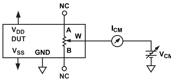
Figure 30. Common-Mode Leakage Current
