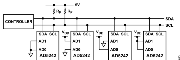
Figure 32. Multiple AD5242 Devices on One Bus
