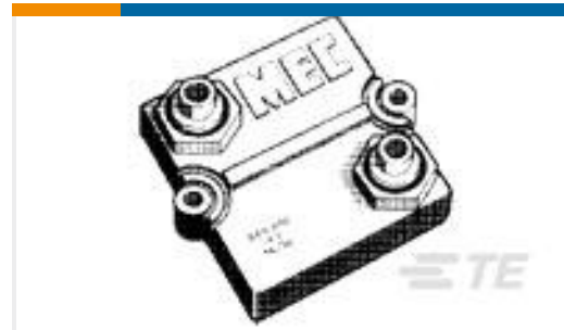
TE Part #1-1614782-4 BDS 2 A 100 470R 10%
