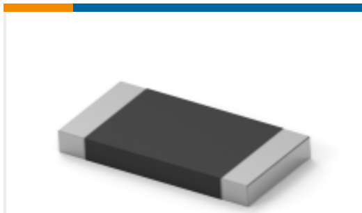
TE Part #8-2176422-7 TLRP 2512 3.0W R025 1% 75PPM 4K RL
