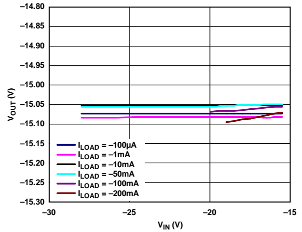
Figure 42. Output Voltage ( V_{OUT} ) vs. Input Voltage ( V_{IN} ), Adjustable Output Voltage, V_{OUT} = -15\text{ V}
