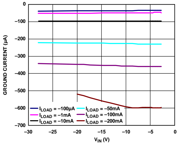
Figure 39. Ground Current vs. Input Voltage ( V_{IN} ), V_{OUT} = -1.22\text{ V}
