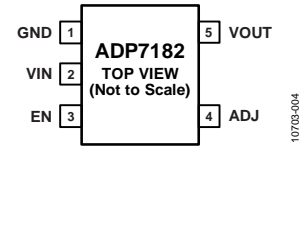
Figure 4. 5-Lead TSOT Pin Configuration, Adjustable Output Voltage
