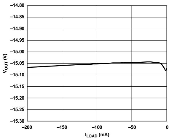
Figure 41. Output Voltage ( V_{OUT} ) vs. Load Current ( I_{LOAD} ), Adjustable Output Voltage, V_{OUT} = -15\text{ V}
