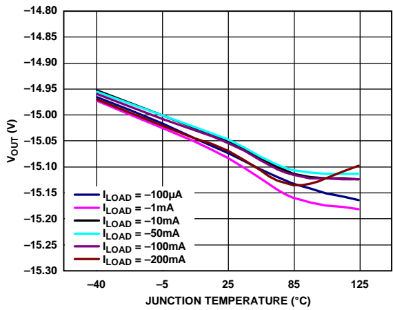
Figure 40. Output Voltage ( V_{OUT} ) vs. Junction Temperature ( T_j ), Adjustable Output Voltage, V_{OUT} = -15\text{ V}
