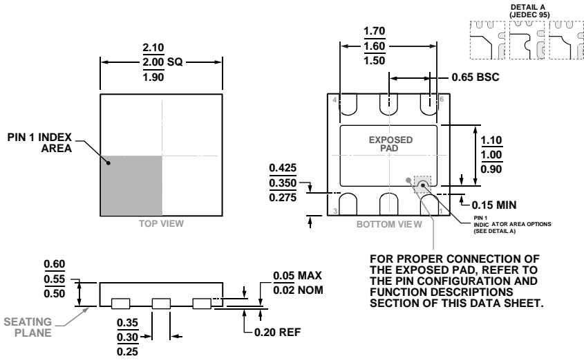
Figure 104. 6-Lead Lead Frame Chip Scale Package [LFCSP] 2.00 mm x 2.00 mm Body and 0.55 Package Height (CP-6-3) Dimensions shown in millimeters
