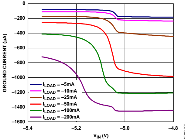
Figure 27. Ground Current vs. Input Voltage ( V_{IN} ) in Dropout, V_{OUT} = -5\text{ V}
