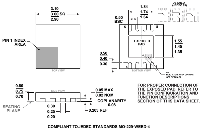
COMPLIANT TO JEDEC STANDARDS MO-229-WEED-4 Figure 105. 8-Lead Lead Frame Chip Scale Package [LFCSP] 3 mm x 3 mm Body and 0.75 Package Height (CP-8-13) Dimensions shown in millimeters
