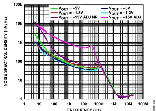
Figure 62. Noise Spectral Density, Various Output Voltages
