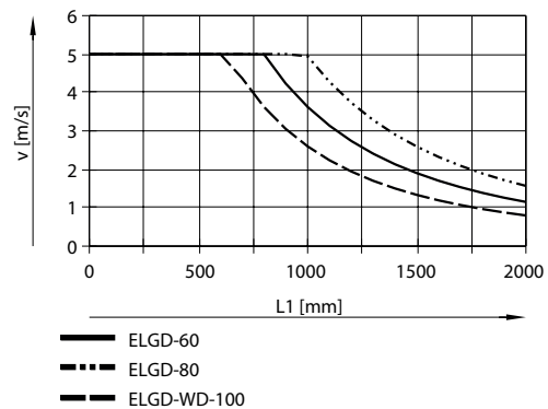
Max. speed v as a function of nominal length L1
