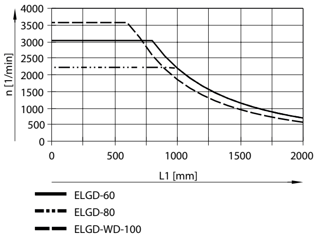
Max. rotational speed n as a function of nominal length L1
