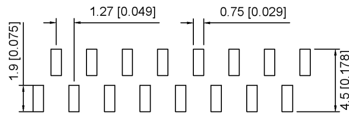
PCB LAYOUT (R2)
