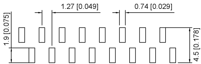
PCB LAYOUT (R1)
