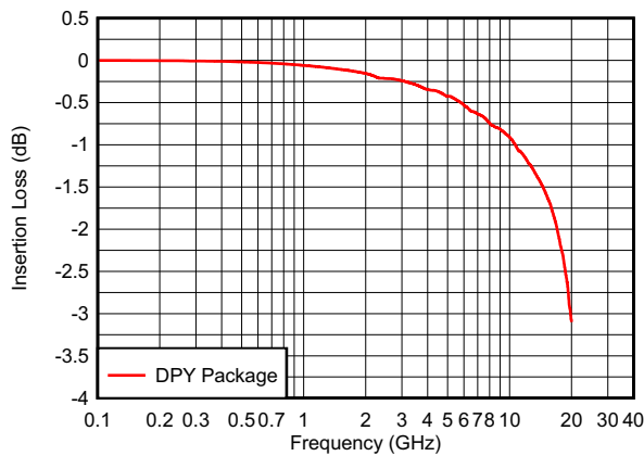
Figure 6-11. Insertion Loss
