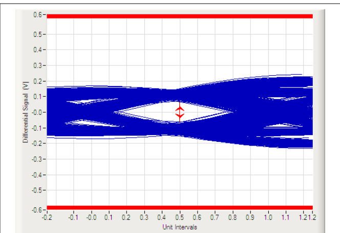
Figure 8-3. USB 3.1 Gen 2 10-Gbps Eye Diagram (with TPD1E01B04-Q1)
