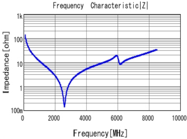
■ GJM1555C1H120FB01 |Z| DC0V, 25degC
