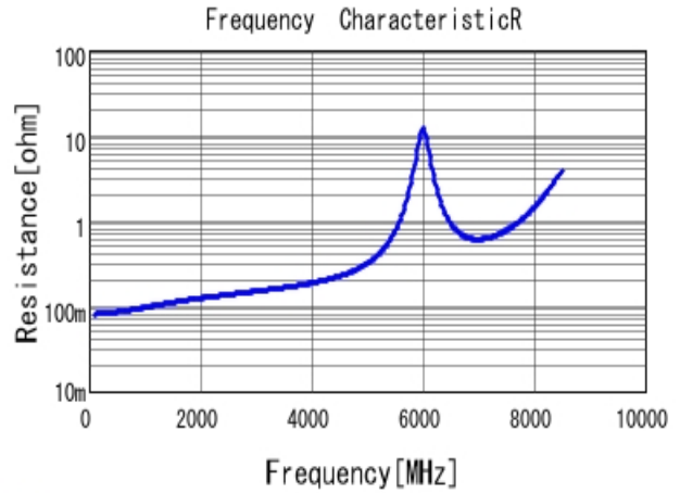
■ GJM1555C1H120FB01 R DC0V, 25degC
