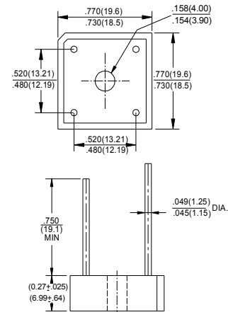
Polarity shown on side of case, Positive lead by beveled corner. Dimensions in inches and (millimeters)
