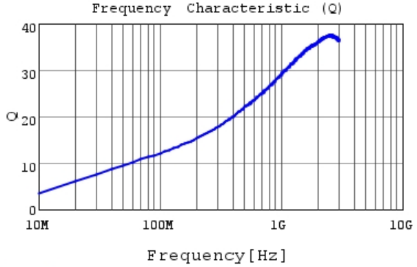
LQP03TN5N1H02 Q
