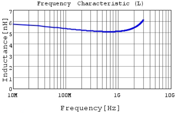
LQP03TN5N1H02 L
