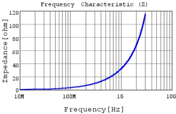
LQP03TN5N1H02 |Z|
