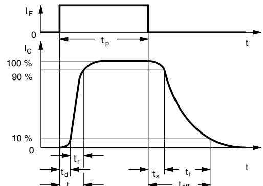
Fig. 4 - Switching Times
