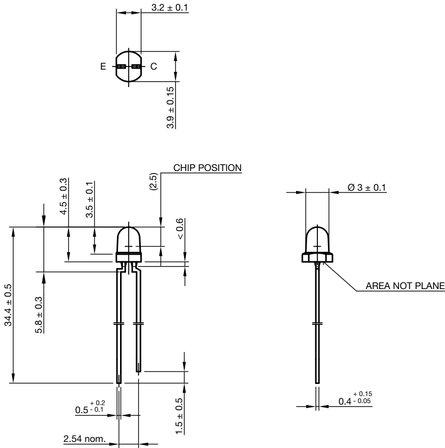
Drawing-No.: 6.544-5269.01-4 Issue: 6; 28.07.14
