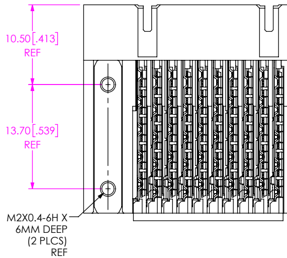
FIG 6 LEFT GUIDANCE EBTF-4-10-2.0-X-RA-X-L-A SHOWN (DIFFERENT AS SHOWN, OTHERWISE SAME AS FIG 5)
