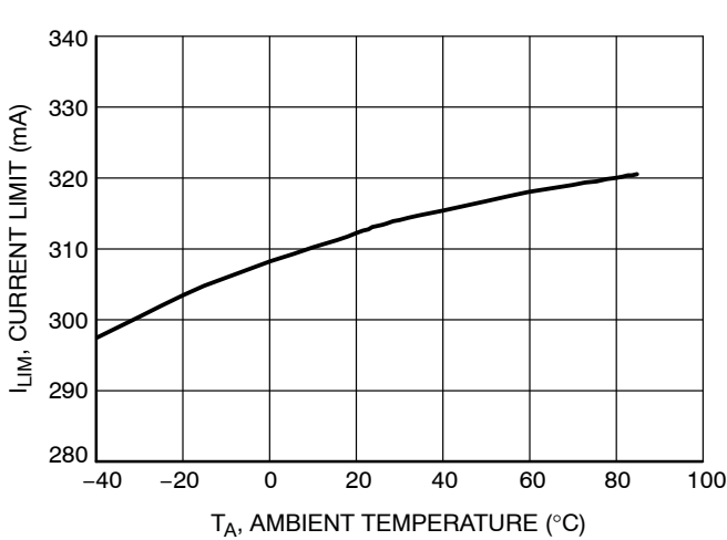
Figure 16. Current Limit vs. Temperature
