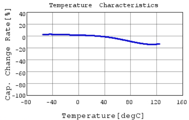
GRM31BR72J103KW01 C-Temp. capchange, DCOV, 1
