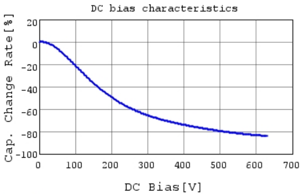
GRM31BR72J103KW01 C-DC bias capchange, 25.0c
