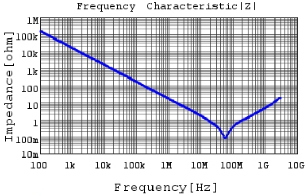
GRM31BR72J103KW01 |Z| DCOV, 25degC
