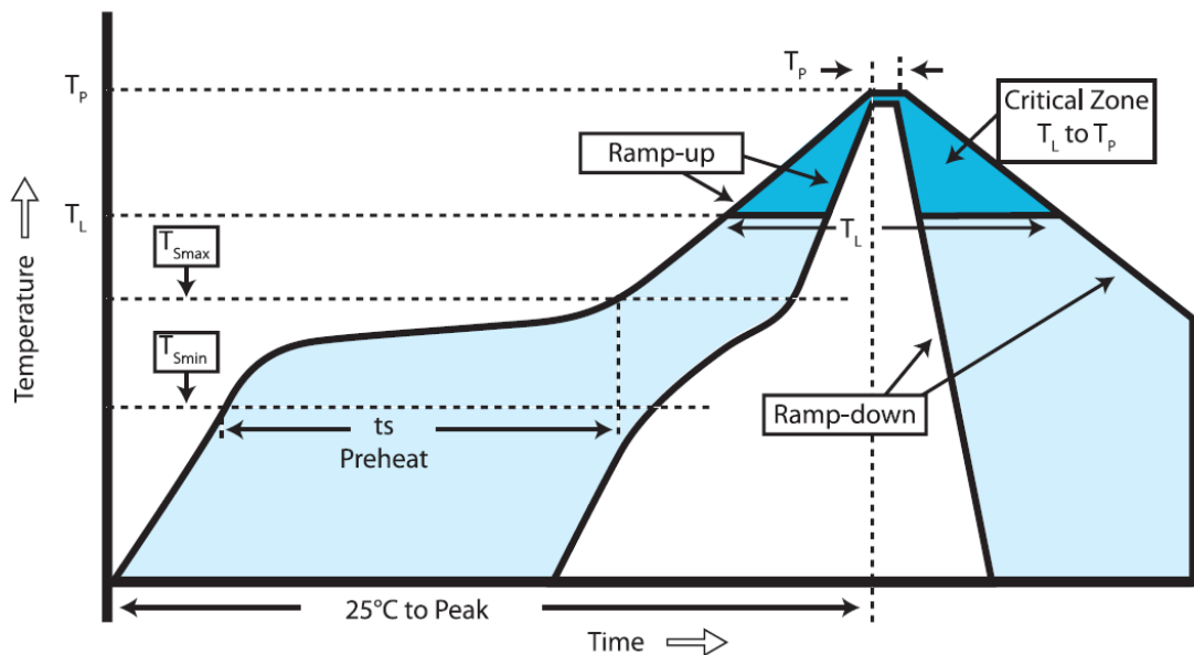
Figure 7. Soldering profile
