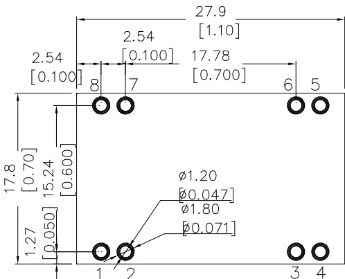
Component-side footprint
