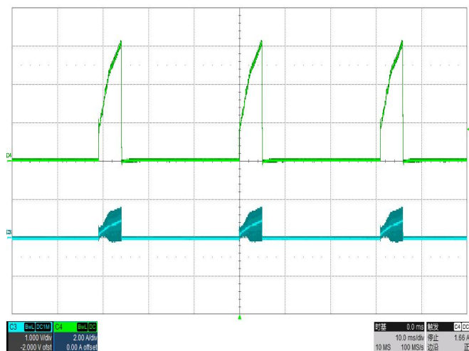
Short-Circuit Output, Vin=36V (C4: Load current)
