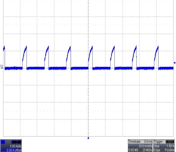
Short-Circuit Output, Vin=48V (C3: Load current)
