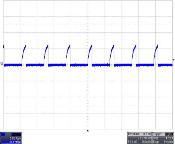
Short-Circuit Output, Vin=40V (C3: Load current)
