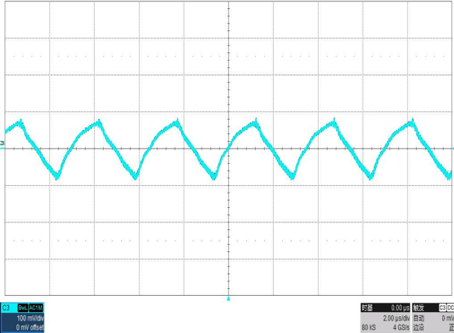
Noise V_{IN}=36V, I_o=1A, 5\sim 20MHz Bandwidth
