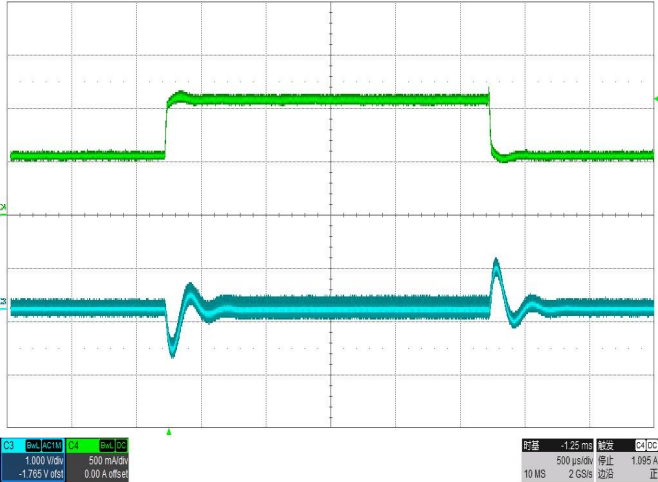
Transient Response, V_{in}=36V, I_o=50\%\sim 100\%\sim 50\% (C3: Output Voltage, C4: Load current)
