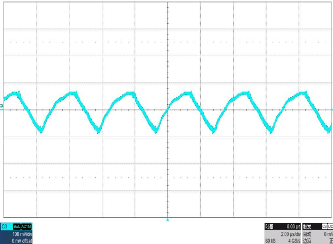
Noise V_{IN}=48V, I_o=1.1A, 5\sim 20MHz Bandwidth
