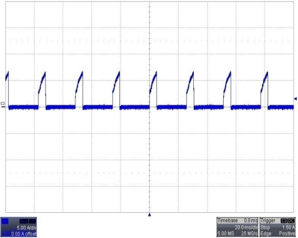
Short-Circuit Output Vin=57V (C3: Load current)
