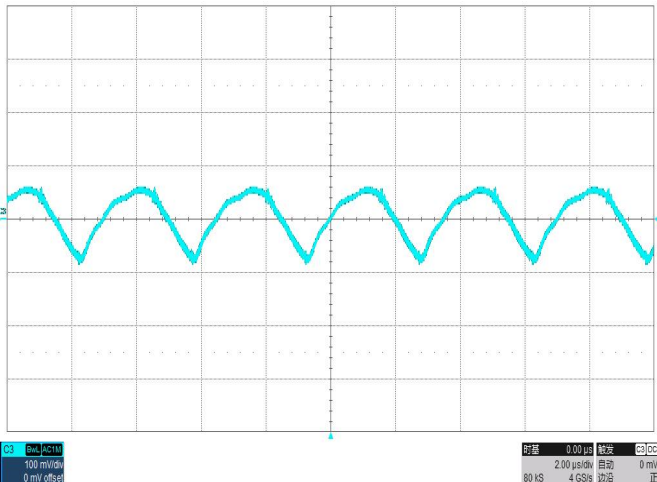
Noise V_{IN}=57V, I_o=1.1A, 5\sim 20MHz Bandwidth
