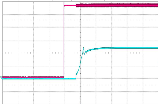
Power Up Vin=48V (C3: output, C2: input)
