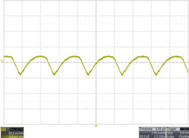
Noise V_{IN}=48V , I_o=2A , 5~20MHz Bandwidth
