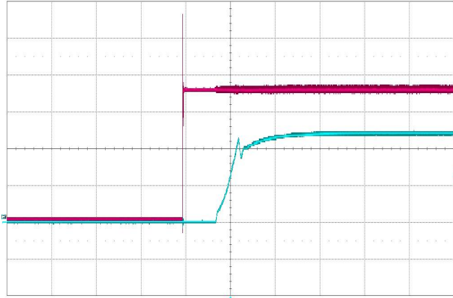
Power Up Vin=36V (C3: output, C2: input)
