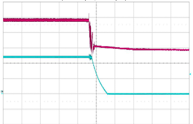
Power Down Vin=36V (C3: output, C2: input)
