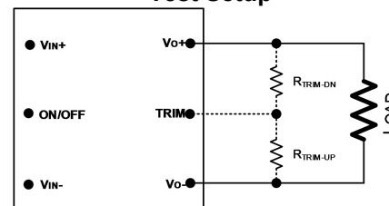
Fig 3. Output Ripple and Noise Test Setup
