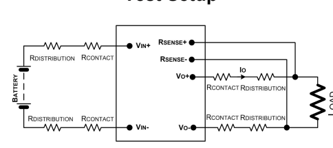
Fig 2. Output Voltage and Efficiency Test Setup
