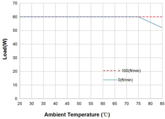
Power Derating
