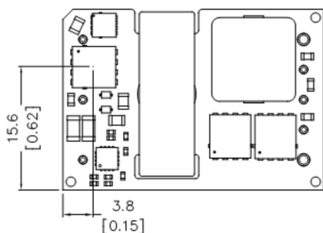
Fig7 Thermal test point(Open Frame Version)
