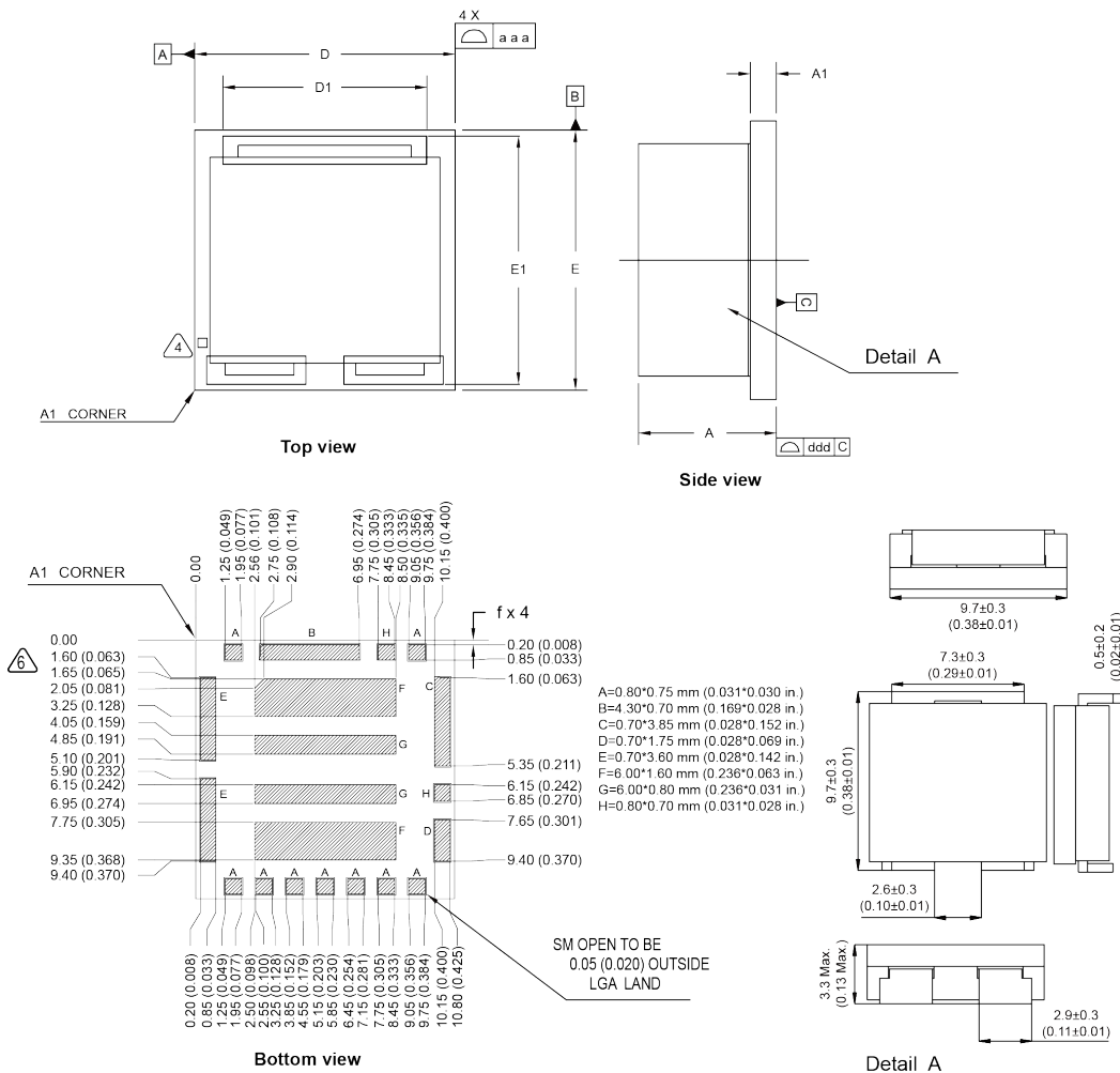
Figure 1-1 Mechanical diagram
