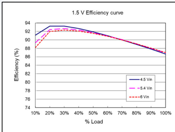
Efficiency curve ( V_{nom} = 5.4\text{ V} , V_{out} = 1.5\text{ V} )
