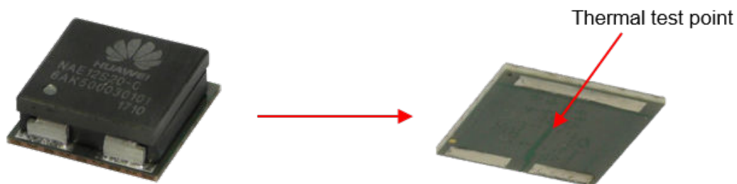
Figure 9-1 Thermal test point
