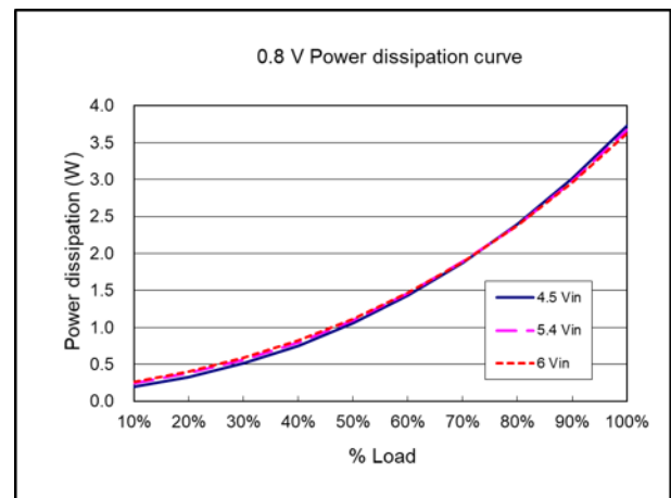
Power dissipation curve ( V_{nom} = 5.4\text{ V} , V_{out} = 0.8\text{ V} )
