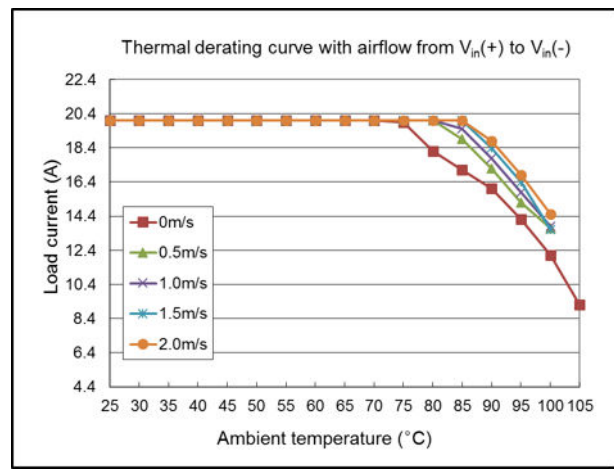
Thermal derating with airflow from V_{in}(+) to V_{in}(-) ( V_{in} = 5.5\text{ V} ; V_{out} = 0.7\text{ V} )
