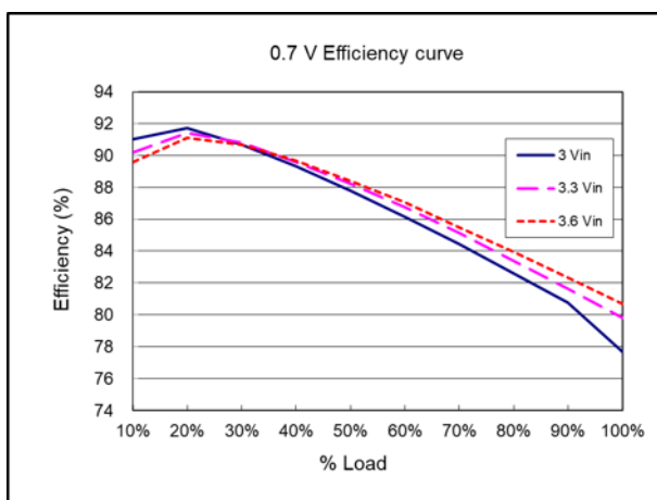
Efficiency curve ( V_{nom} = 3.3\text{ V} , V_{out} = 0.7\text{ V} )
