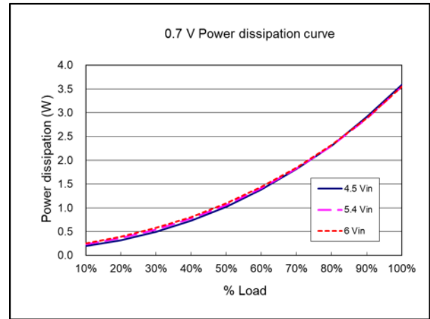
Power dissipation curve ( V_{nom} = 5.4\text{ V} , V_{out} = 0.7\text{ V} )
