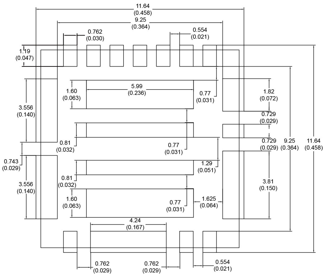
Figure 10-1 Encapsulation Size Diagram
