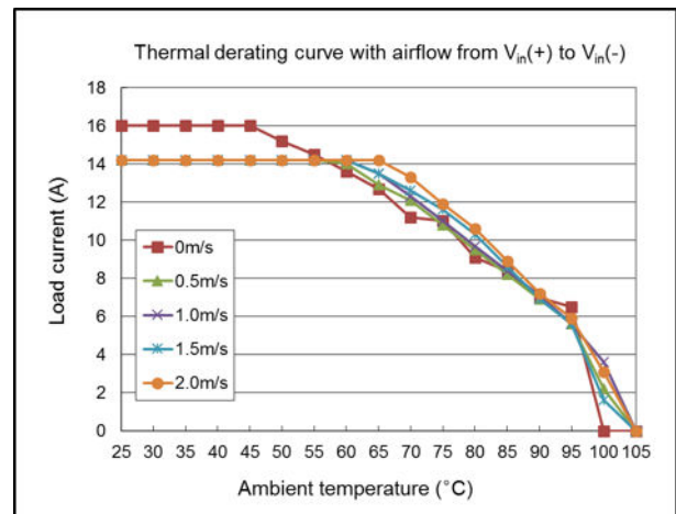
Thermal derating with airflow from V_{in}(+) to V_{in}(-) ( V_{in} = 12\text{ V} ; V_{out} = 5.5\text{ V} )
