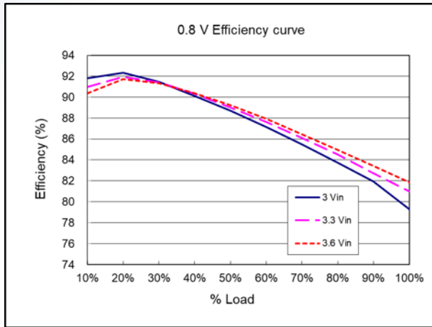
Efficiency curve ( V_{nom} = 3.3 V , V_{out} = 0.8 V )
