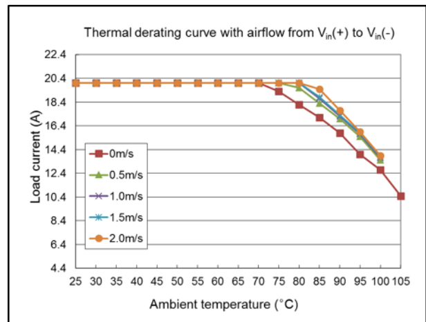
Thermal derating with airflow from V_{in}(+) to V_{in}(-) ( V_{in} = 3.3\text{ V} ; V_{out} = 0.8\text{ V} )
