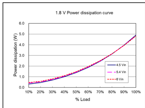
Power dissipation curve ( V_{nom} = 5.4\text{ V} , V_{out} = 1.8\text{ V} )
