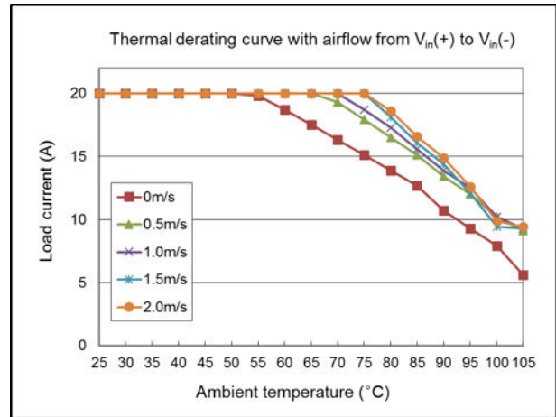
Thermal derating with airflow from V_{in}(+) to V_{in}(-) ( V_{in} = 12\text{ V} ; V_{out} = 0.7\text{ V} )
