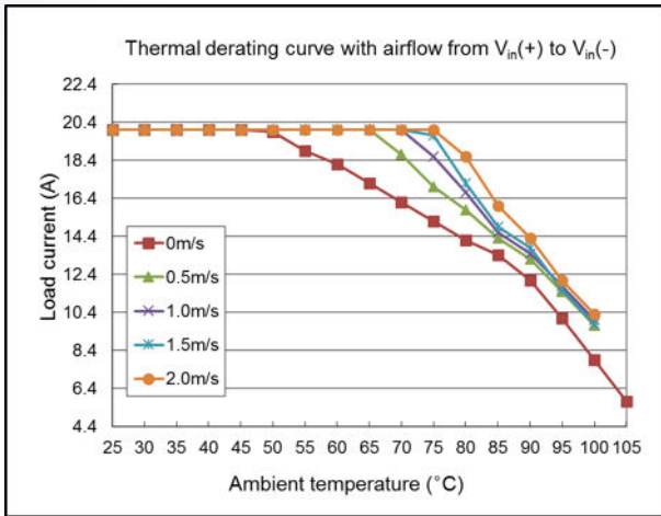
Thermal derating with airflow from V_{in}(+) to V_{in}(-) ( V_{in} = 5.5\text{ V} ; V_{out} = 2.1\text{ V} )
