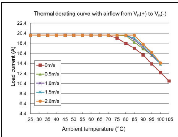
Thermal derating with airflow from V_{in}(+) to V_{in}(-) ( V_{in} = 3.3\text{ V} ; V_{out} = 0.7\text{ V} )
