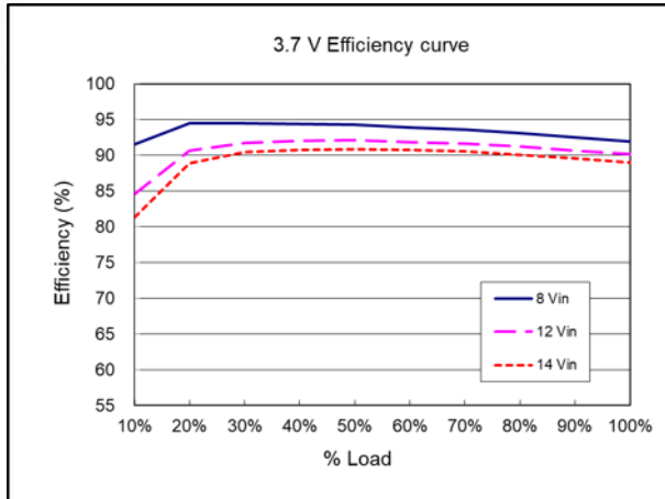
Efficiency curve ( V_{nom} = 12.0\text{ V} , V_{out} = 3.7\text{ V} )
