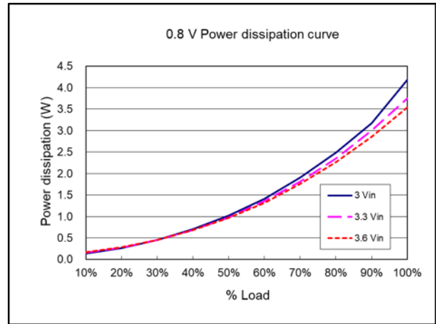
Power dissipation curve ( V_{nom} = 3.3 V , V_{out} = 0.8 V )
