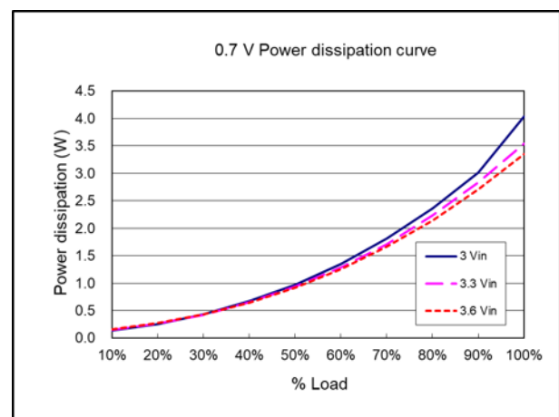
Power dissipation curve ( V_{nom} = 3.3\text{ V} , V_{out} = 0.7\text{ V} )
