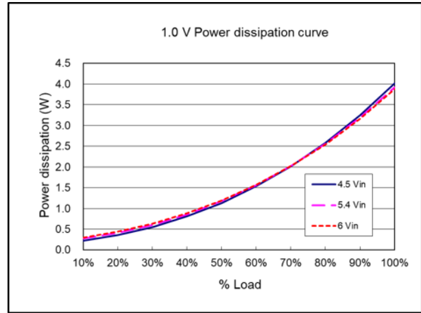
Power dissipation curve ( V_{nom} = 5.4\text{ V} , V_{out} = 1.0\text{ V} )
