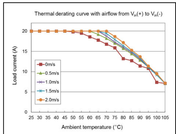
Thermal derating with airflow from V_{in}(+) to V_{in}(-) ( V_{in} = 12\text{ V} ; V_{out} = 0.9\text{ V} )
