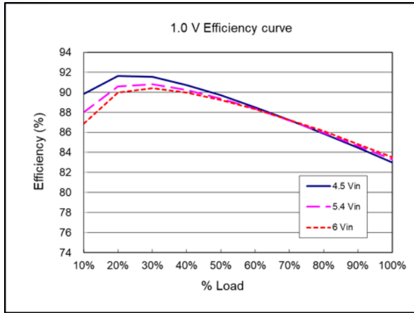
Efficiency curve ( V_{nom} = 5.4\text{ V} , V_{out} = 1.0\text{ V} )
