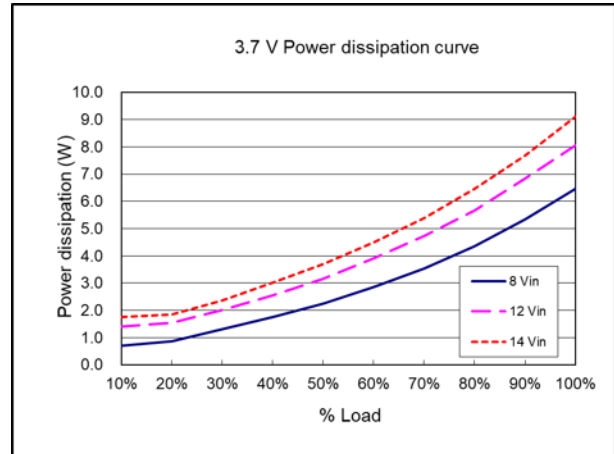
Power dissipation curve ( V_{nom} = 12.0\text{ V} , V_{out} = 3.7\text{ V} )
