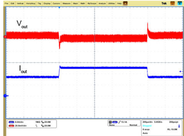
Load: 50%–75%–50%, di/dt = 5 \text{ A}/\mu\text{s}
