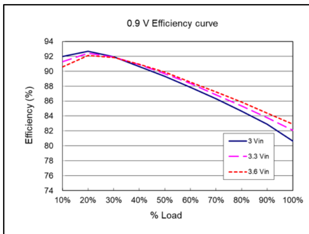
Efficiency curve ( V_{nom} = 3.3 V , V_{out} = 0.9 V )
