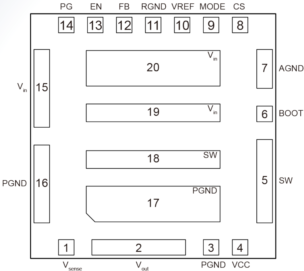
Figure 1-2 Pin Description
