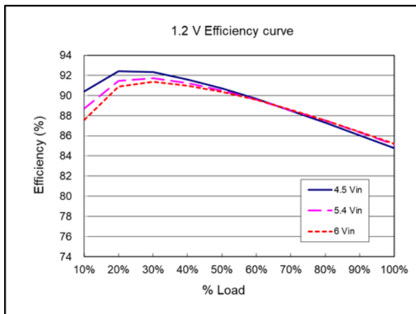
Efficiency curve ( V_{nom} = 5.4\text{ V} , V_{out} = 1.2\text{ V} )
