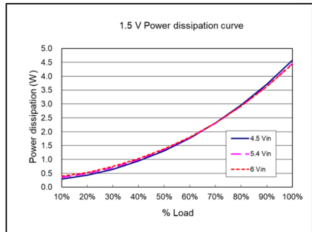
Power dissipation curve ( V_{nom} = 5.4\text{ V} , V_{out} = 1.5\text{ V} )
