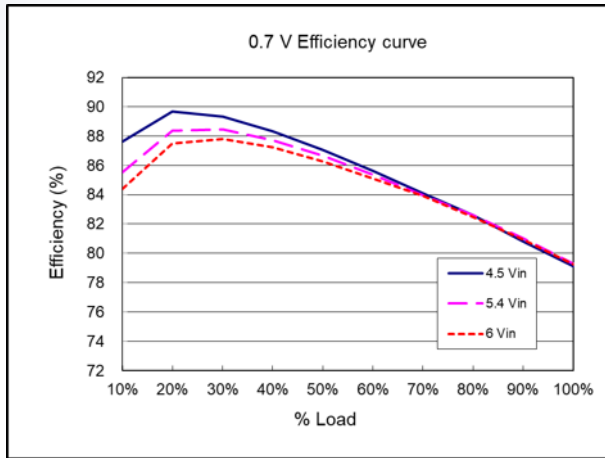
Efficiency curve ( V_{nom} = 5.4\text{ V} , V_{out} = 0.7\text{ V} )
