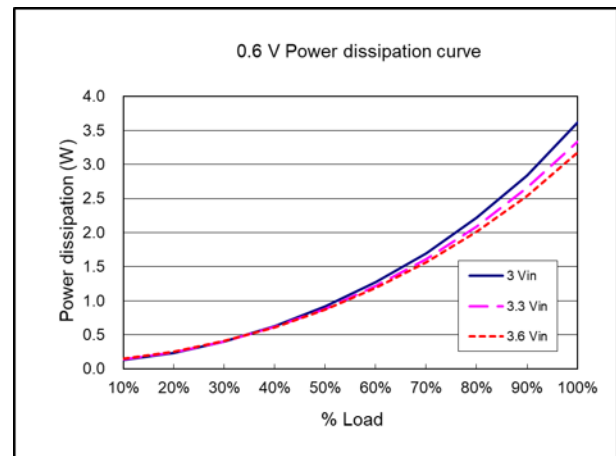
Power dissipation curve ( V_{nom} = 3.3\text{ V} , V_{out} = 0.6\text{ V} )
