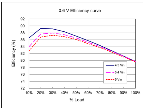
Efficiency curve ( V_{nom} = 5.4\text{ V} , V_{out} = 0.6\text{ V} )
