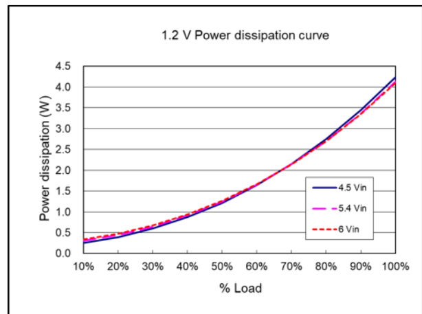
Power dissipation curve ( V_{nom} = 5.4\text{ V} , V_{out} = 1.2\text{ V} )
