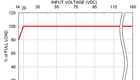
QAE100-72S□□U Derating Curve vs. Input Voltage
