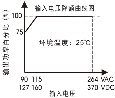
LOF450-20Bxx 输入电压降额
