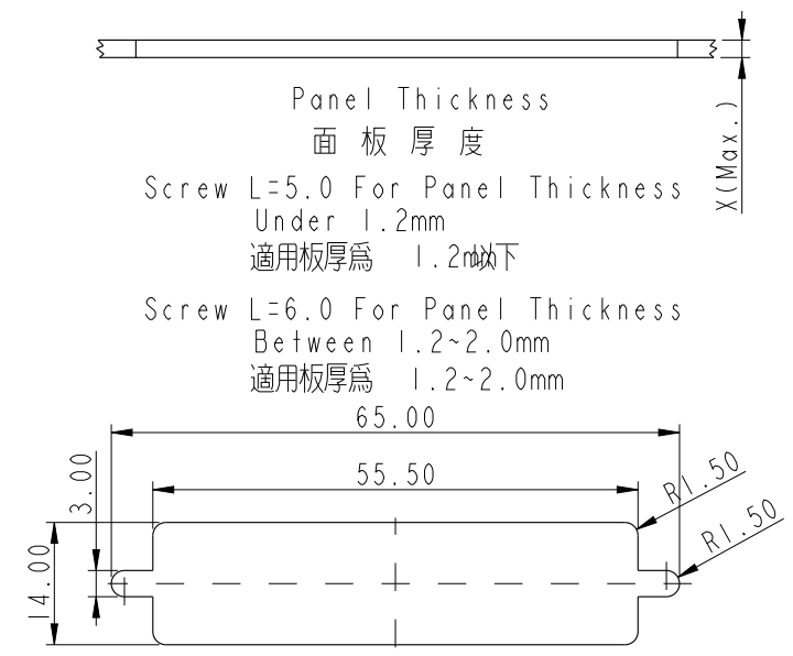
Recommended Panel Cut-Out 建議挖孔尺寸
